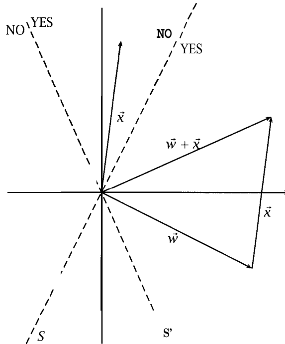
Figure 16.8 One error-correcting step of the perceptron learning algorithm. Data vector \vec{x} is misclassified by the current weight vector \vec{w} since it lies on the no -side of the decision boundary S . The correction step adds \vec{x} to \vec{w} and (in this case) corrects the decision since \vec{x} now lies on the yes -side of S , the decision boundary of the new weight vector \vec{w} + \vec{x} .
