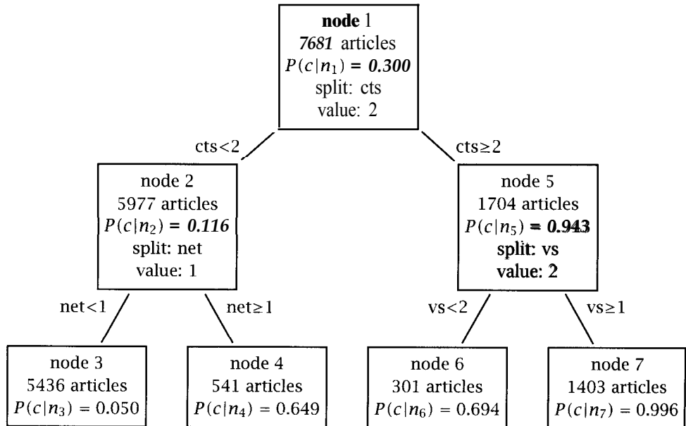
Figure 16.1 A decision tree. This tree determines whether a document is part of the topic category earnings or not. P(c|n_i) is the probability of a document at node n_i to belong to the earnings category c .
